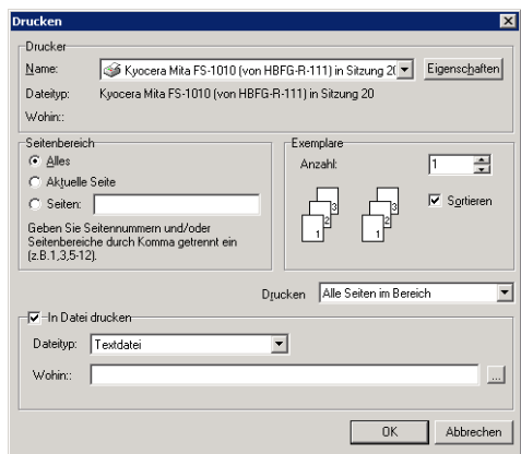
Abb. 4-2: Report-Druck
